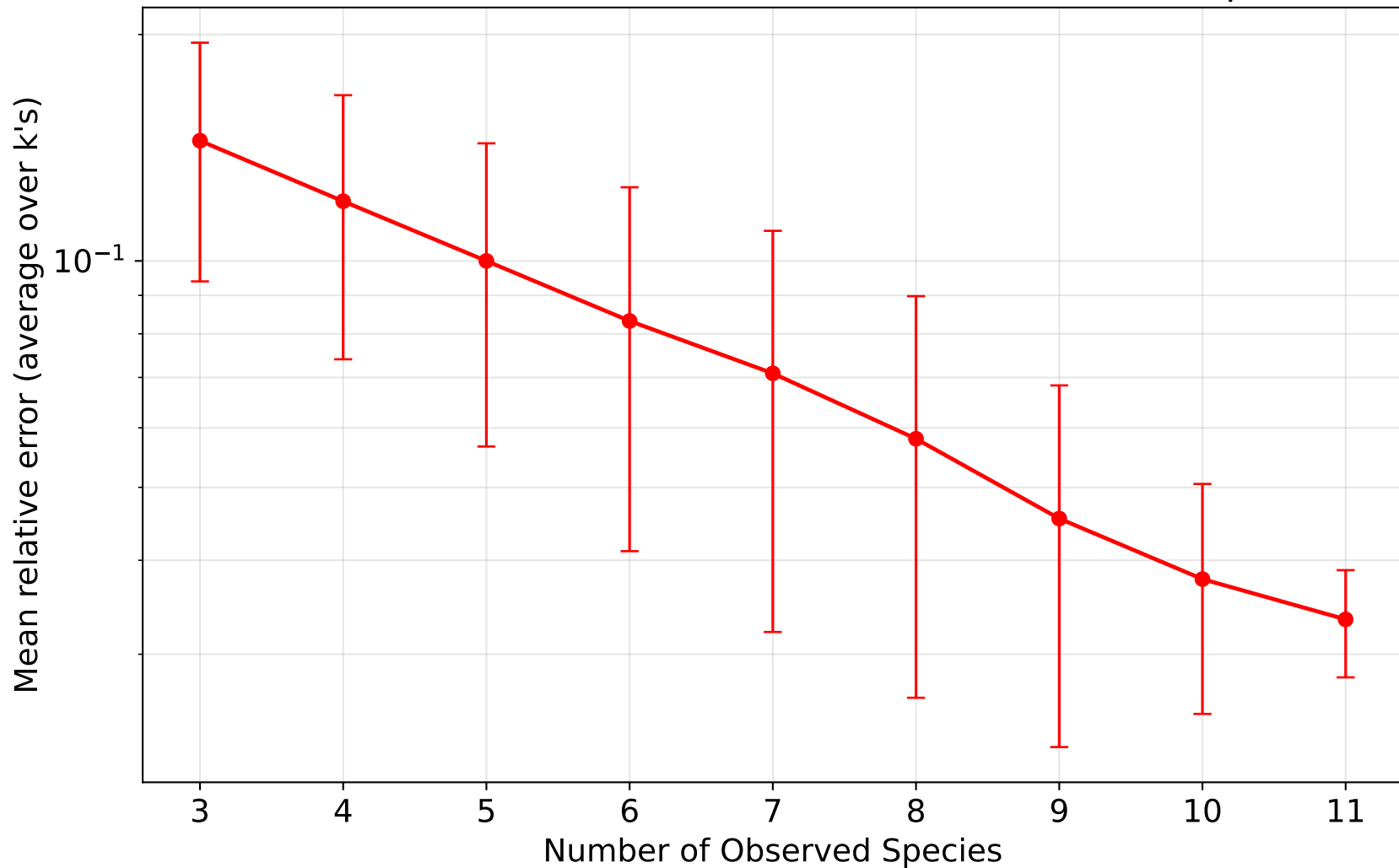
50, 50 — Mean relative error vs number of observed species
